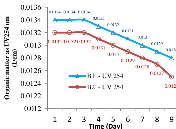
Figure 6) Changes in UV254 during 9 days for open lid (B1) and closed lid (B2) at the end of water network.
